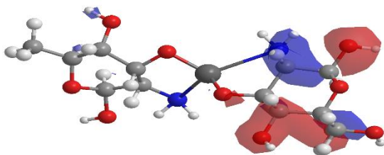
LUMO (N=77) [-9,441 eV]
