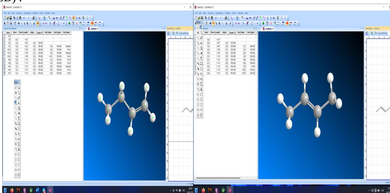
2-rasm. Alkenlarning ( Buten-1 va buten-2 ning) 3D formulalari
