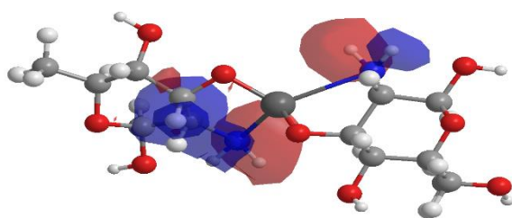
LUMO (N=77) [-9,441 eV]
