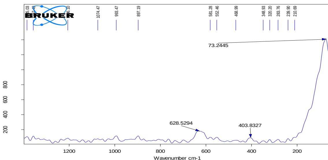
2-rasm. Ba 2 Sr 2 CaCu 2 O x ning Raman spektri
