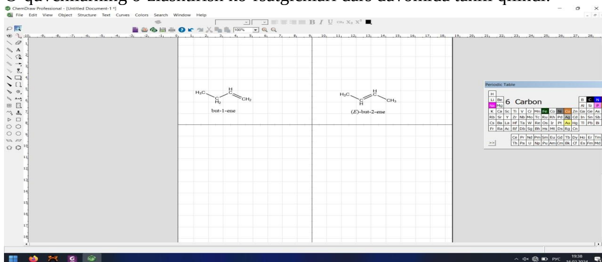
1-rasm. ChemDraw dasturida alkenlarning tuzilish formulalarini yozish.
