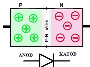
1-rasm. To'g'rilovchi diodlar
