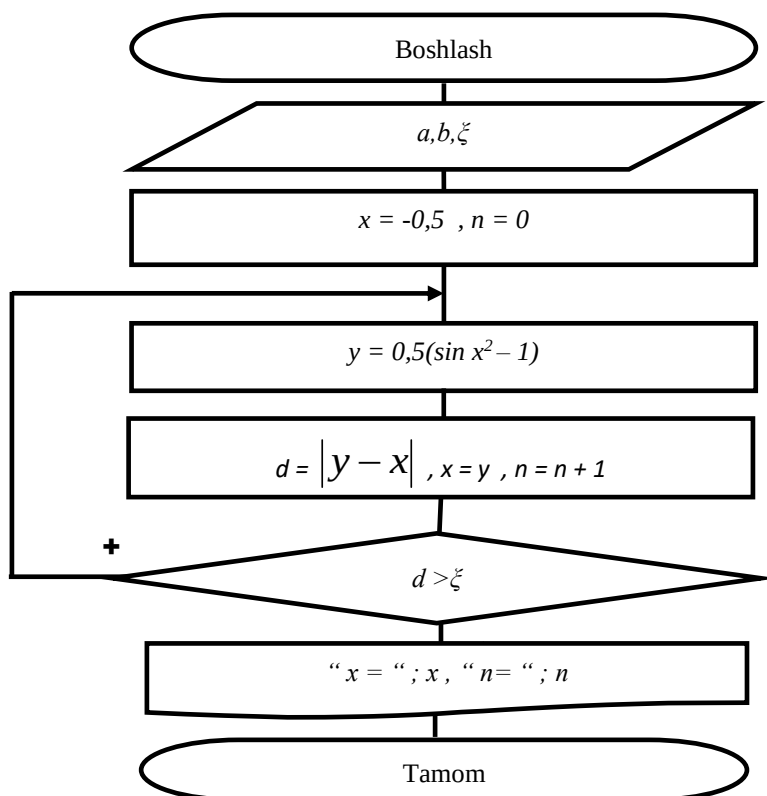
5-rasm. Iteratsiya usulining blok sxemasi
