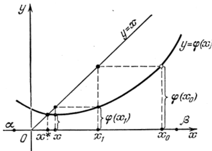
4-rasm. Iteratsiya metodining geometrik ko‘rinishi
