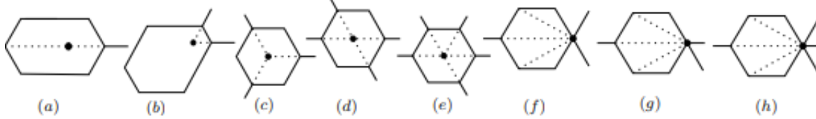
Fig 1. All possible self-shrinker with one bounded phase.
