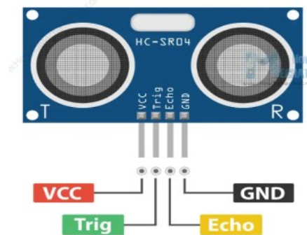
2-rasm. Ultrasonik sensorning pinlari.
