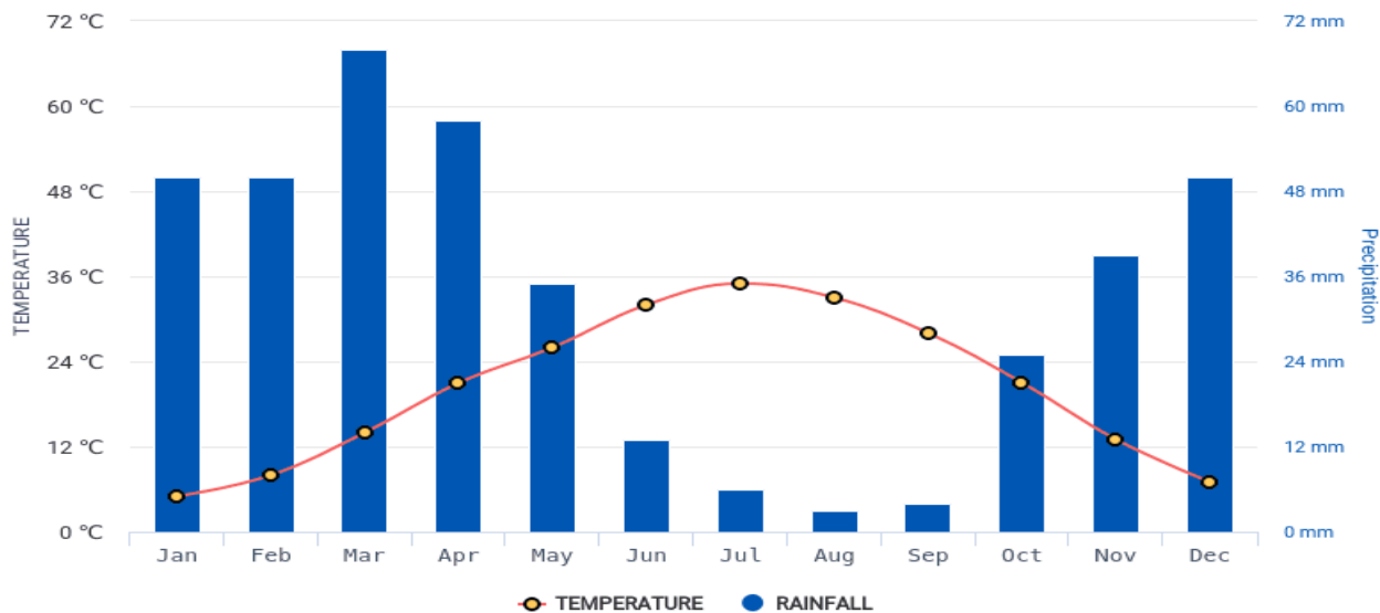
Figure 5. General temperature and precipitation indicators of Tashkent city
