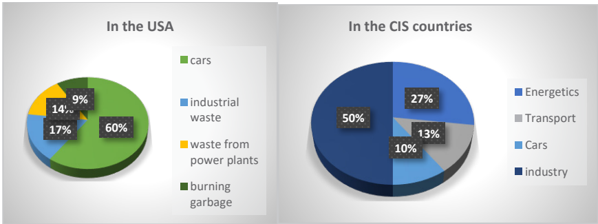
Fig. 1. "Sources of atmospheric pollution"
